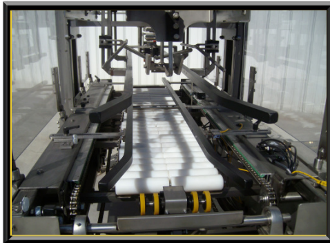
Case Indexer with Speed Up Wheels
